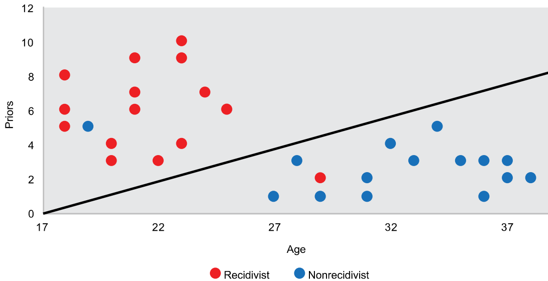
Figure 1: Simple Decision Boundary
