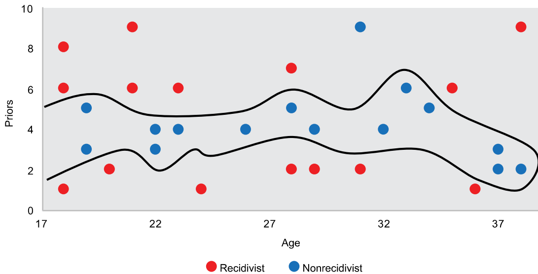
Figure 2: Complex Decision Boundary
